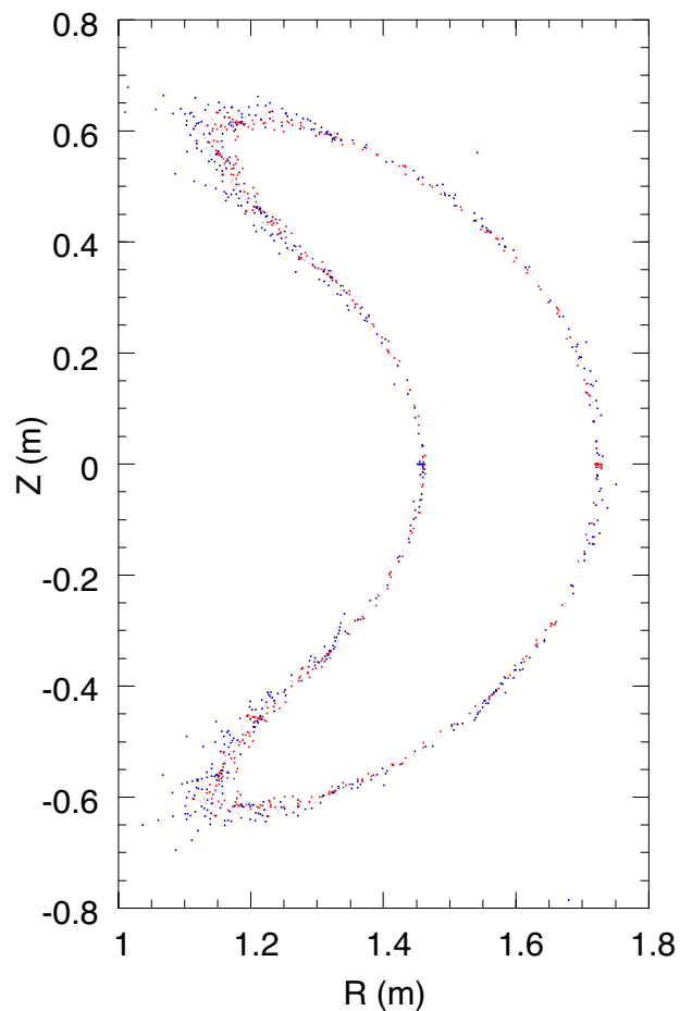
FIG. 7 Poincaré plots of scrapeoff field lines started at the inboard and outboard midplane within 0-1 cm of the nominal (VMEC) boundary and followed for 20 toroidal revolutions.
