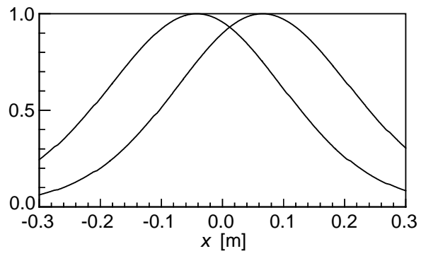
FIG. 9. Same as in case a ) of Fig. 8 but with the opposite value of launching angle ( \gamma = 4.5^\circ ).
