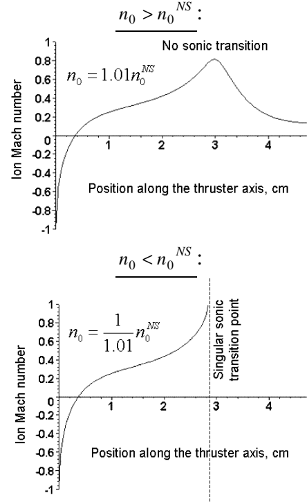
FIG. 1. Types of the ion velocity spatial behavior for different values of the plasma density at the anode. Case T_e = Const T
