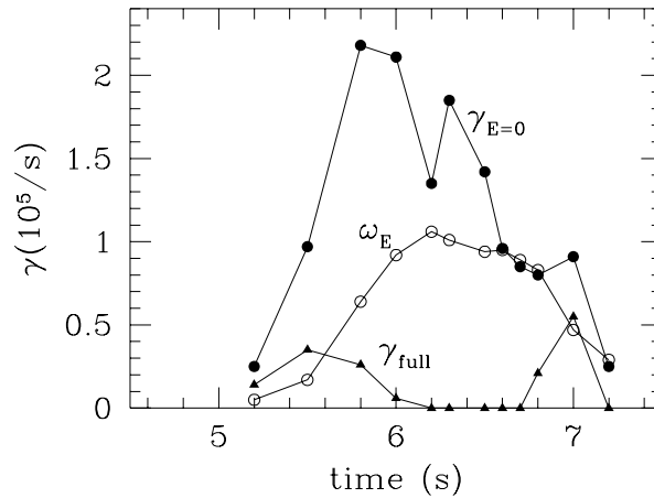
Fig. 4. Growth rates and shearing rates vs. time at the \rho = 0.4 surface, calculated with and without \mathbf{E} \times \mathbf{B} shear. At t = 6 s the shearing rate has increased to within a factor of 2 of the linear growth rate ignoring \mathbf{E} \times \mathbf{B} shear, \gamma_{E=0} . Later, toroidal rotation slows and \omega_E drops below \gamma_{E=0} . The full linear growth rates including \mathbf{E} \times \mathbf{B} shear, labelled \gamma_{\text{full}} , correlate well with the reduction in \chi_i as the barrier is formed, and the increase in \chi_i as the barrier collapses.
