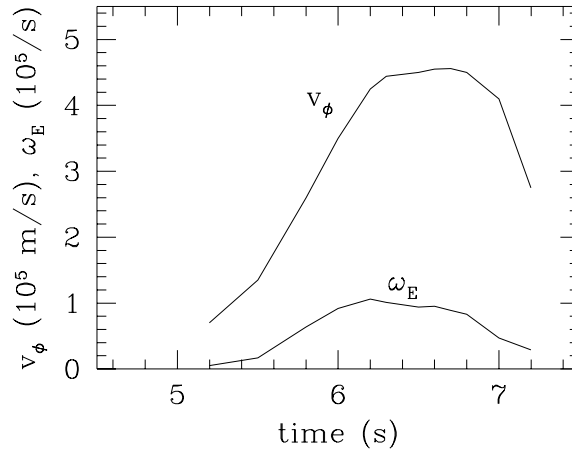
Fig. 3. Toroidal rotation at R = 340cm , v_\phi , and the shearing rate at \rho = 0.4 , \omega_E , vs. time. After t = 6.8s , core rotation slows and \omega_E drops.
