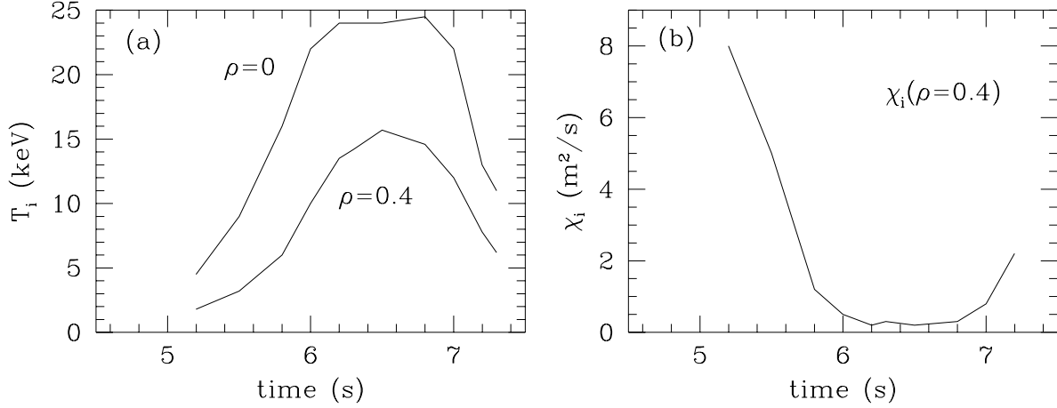
Fig. 2. (a) T_i and (b) \chi_i(\rho = 0.4) for a JET optimized shear discharge. At t = 6.8s the core ITB collapses.
