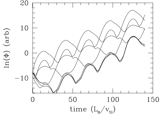
Fig. 1. \Phi(t) for seven \theta'_0 's in the presence of \mathbf{E} \times \mathbf{B} shear. In this representation the addition of flow shear introduces oscillations on top of exponential growth, and a reduced effective growth rate.
