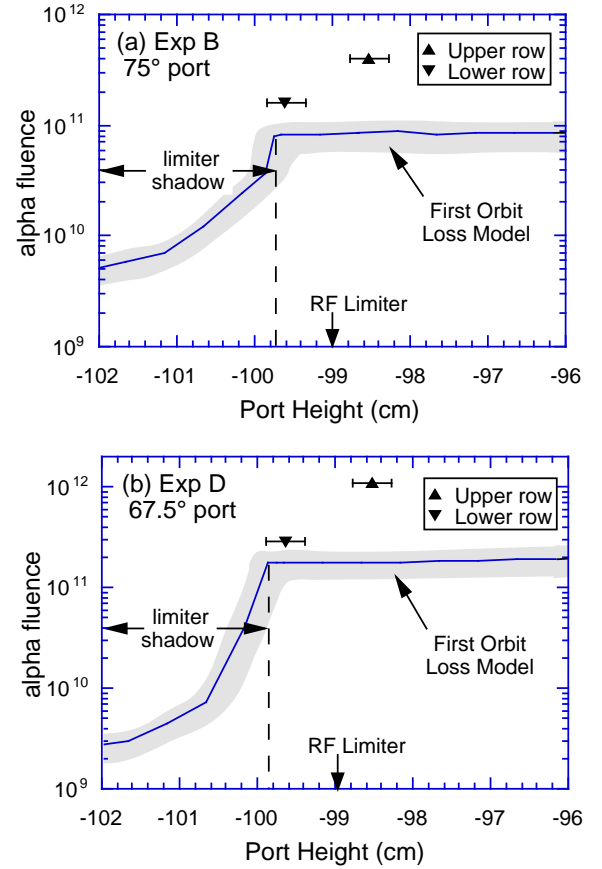
FIG. 20. I_p = 1.8 MA - Alpha fluence for layers 4 through 9 as a function of port height for the upper and lower rows of the (a) 75^\circ port of exposure B, and (b) 67.5^\circ port of exposure D. The RF limiter shadow begins only \sim 2 mm below the midplane of the lower row, possibly placing the lower row partially in the shadow. The decrease in the anomalous loss from the upper to lower row may be attributable to shadowing and/or a radial diffusive loss.
