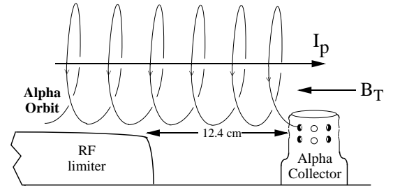
FIG. 3. Side view (looking in toward centerline of TFTR) of the alpha collector probe head depicting a co-going alpha particle entering one of the 16 collimating ports.
