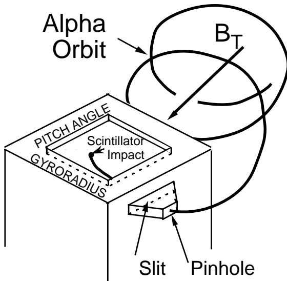
FIG. 5. Schematic diagram of the lost alpha scintillator detector located 90^\circ below the outer midplane. The escaping alphas enter a pair of apertures that disperse them in pitch angle and gyroradius. The 2-D image of the visible light emission from the scintillation screen is transmitted through a quartz fibreoptic bundle to a gated intensified video camera for analysis.
