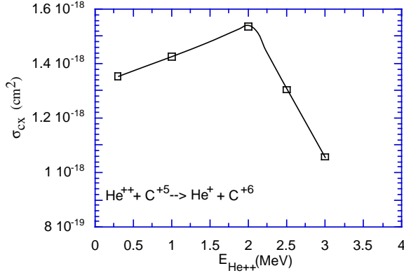
FIG. 22. Calculated single electron capture cross section for the \text{He}^{++} + \text{C}^{+5} collision system.
