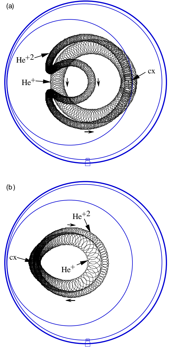
FIG. 24. 2.5 MeV alpha orbit transitions in R = 2.45 m, I_p = 1.8 MA plasmas for alphas charge exchanging (cx) at (a) the outer-midplane crossing point of the co-going leg of a trapped particle ( R = 320 cm, \chi_t = 124^\circ ), and (b) the inner-midplane crossing point of a counter-going passing particle ( R = 200 cm, \chi_t = 70^\circ ), both resulting in inwards radial transport.
