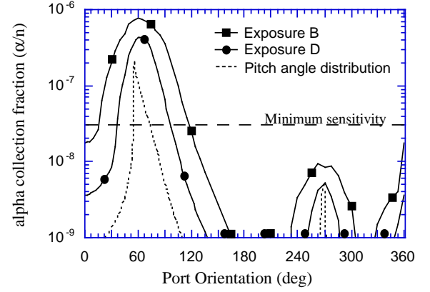
FIG. 6. Predicted alpha collection fraction (alphas/neutron) as a function of port orientation for the 1.8 MA exposures using the original (exposure B) and the redesigned probe head (exposure D). The dashed curve represents the expected pitch angle distribution in arbitrary units. The horizontal dashed line at 3 \times 10^{-8} alphas/neutron represents the minimum sensitivity assuming 1 \times 10^{17} global neutron production.
