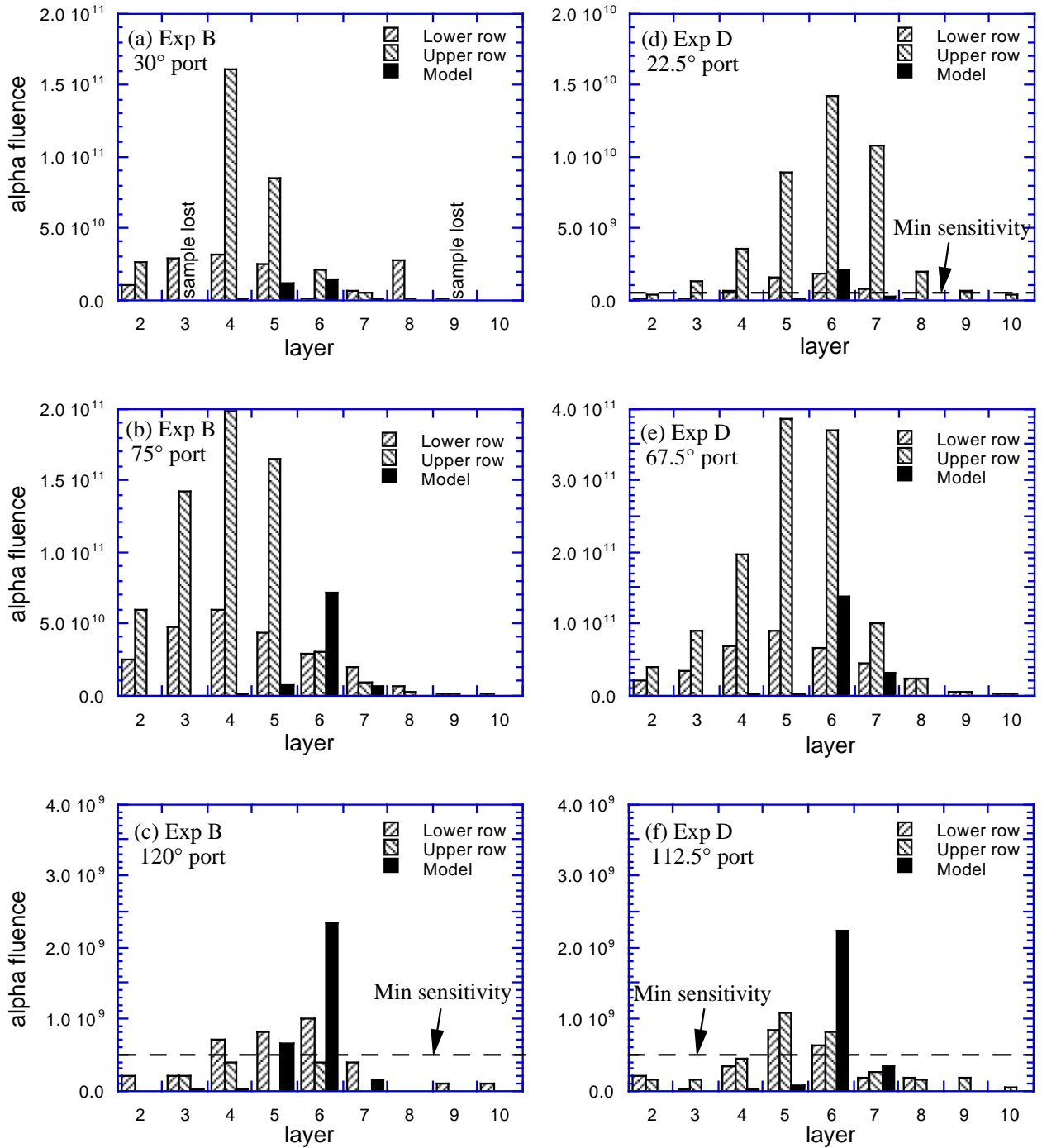
FIG. 13. I_p = 1.8 MA - Implantation range distributions as a function of layer for the upper and lower rows and model predictions for (a) 30^\circ (b) 75^\circ and (c) 120^\circ ports of exposure B, and (d) 22.5^\circ (e) 67.5^\circ and (f) 112.5^\circ ports of exposure D. Same notation as Fig. 12. Layers 3 and 9 of the upper row of the 30^\circ port of exposure B in (a) were lost during the tritium decontamination process [9].
