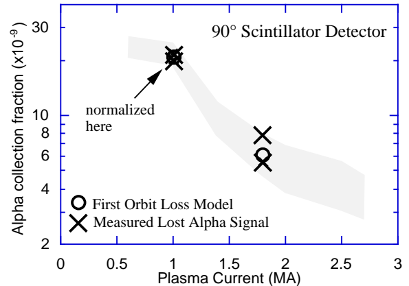
FIG. 11. Plasma current dependence of the alpha collection fraction measured with the 90° lost alpha scintillator detector normalized to the first orbit loss model at 1.0 MA. The shaded region corresponds to the first orbit loss model calculated for R = 2.52 m plasmas in Ref. [1], but appears to fit the R = 2.45 m data well. The good agreement with the model implies that this detector does not ‘see’ the anomalous loss apparent at 1.8 MA using the alpha collector probe.
